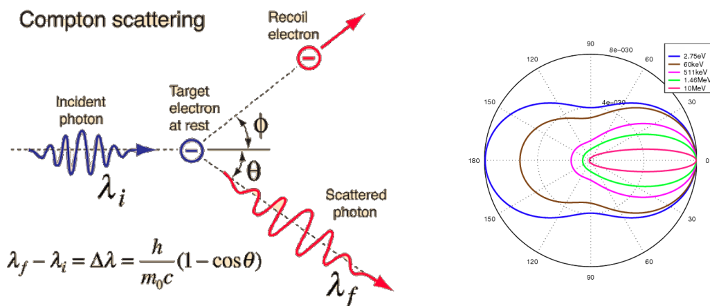
Left: Schematics of a Compton scattering Right: Iso-contours of the Klein-Nishina cross section.
